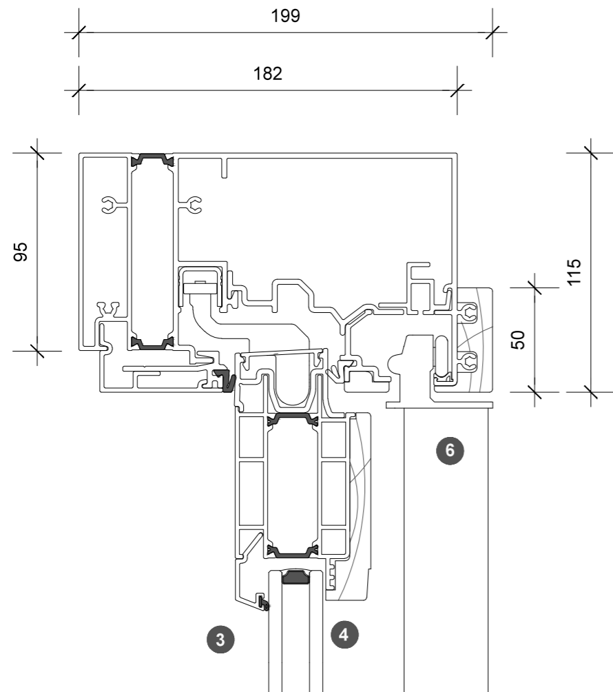
4. head detail
